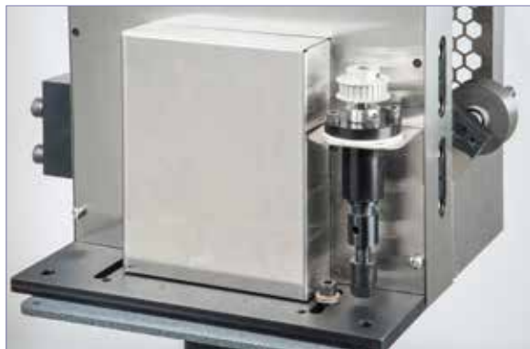
Direct mode (rear view) with transfer roll assembly detached
