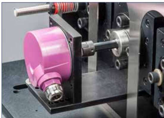
Shown with bracket and coupling for 6mm shaft encoder
